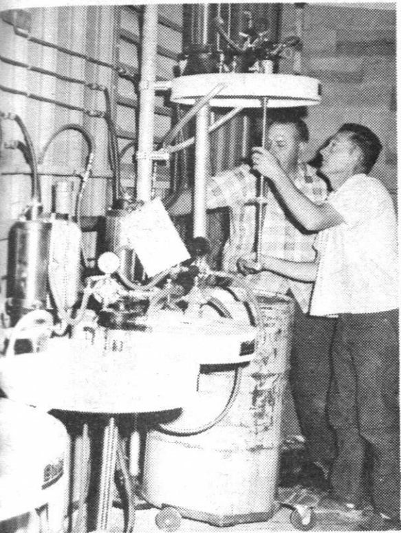
MIXING—This process is carried out in a separate building from the main plant for safety purposes.
